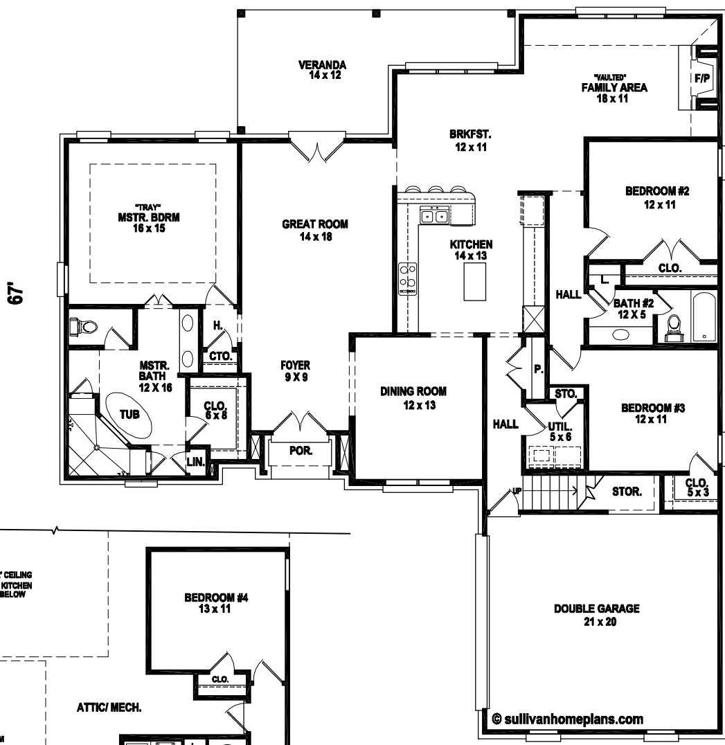
61' FIRST LEVEL FLOOR PLAN
