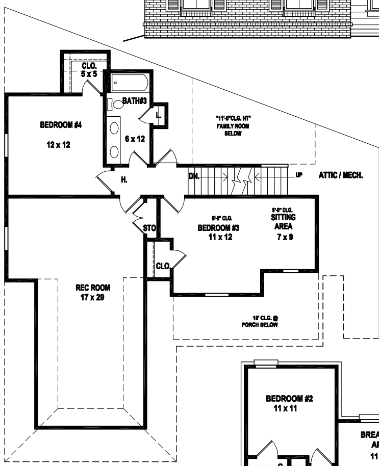
SECOND LEVEL FLOOR PLAN
