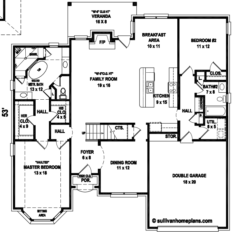
FIRST LEVEL FLOOR PLAN
