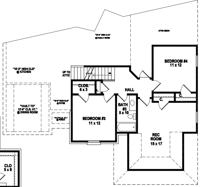
SECOND LEVEL FLOOR PLAN
