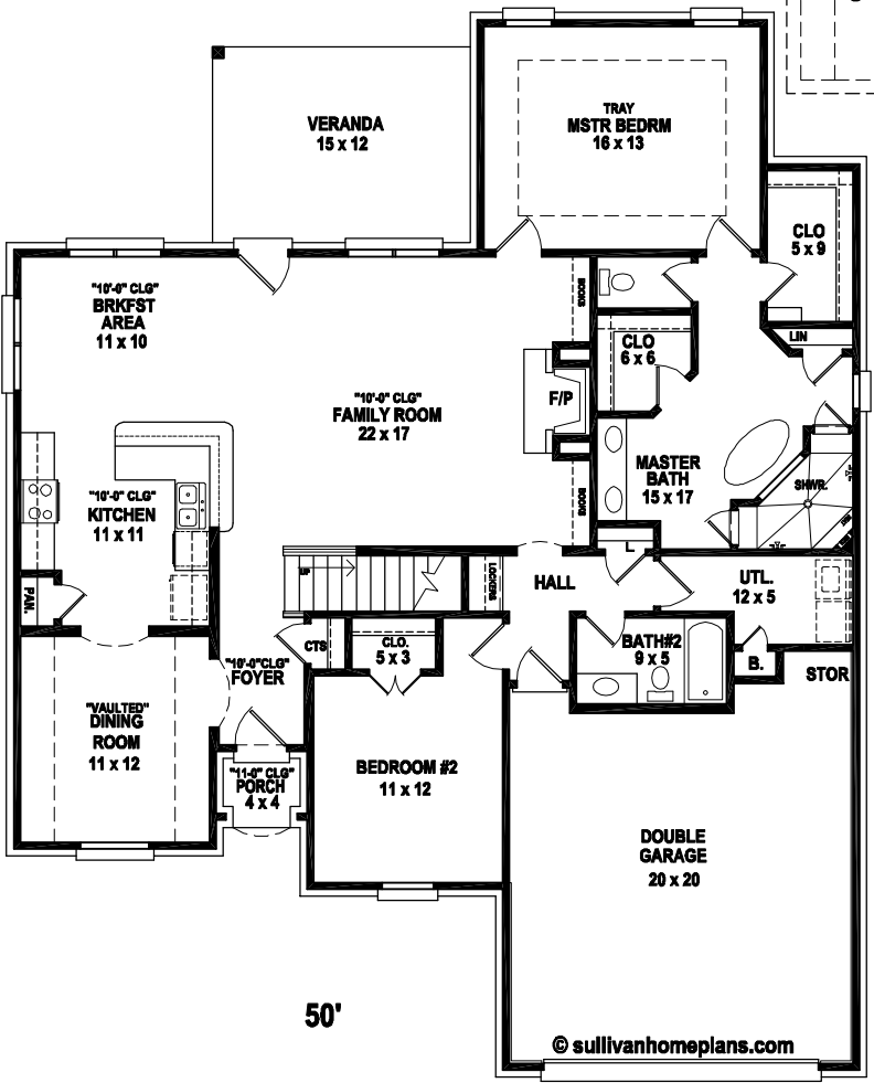
FIRST LEVEL FLOOR PLAN
